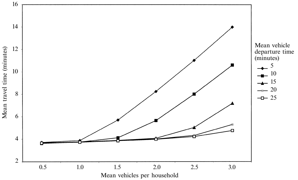
Figure 5. Mean vehicle evacuation travel time.
